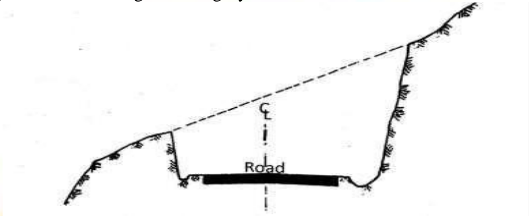
Typical Cross Sections of Box cutting
