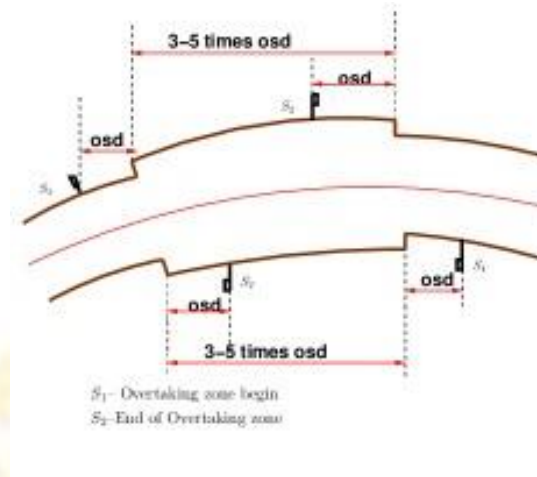
Figure : Overtaking zones
