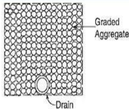
Fig. Geosynthetic-encased aggregate drain with a pipe
