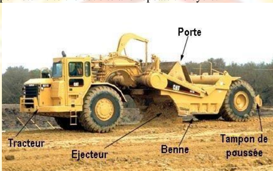
Fig. Scraper
