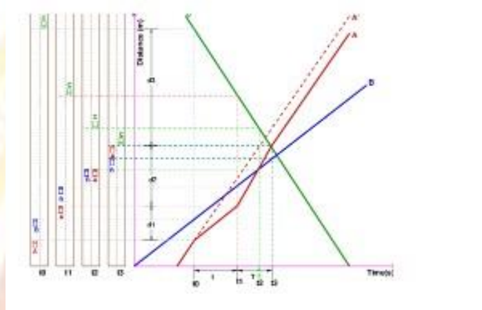
Figure : Time-space diagram: Illustration of overtaking sight distance
