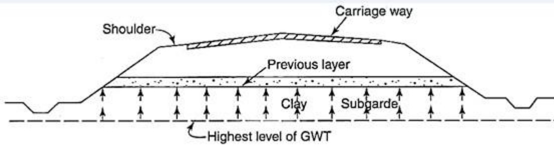
Fig. Capillary cut-off for a clayey subgrade
